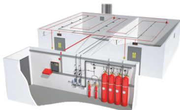
FIRE PROTECTION SYSTEM FOR THE INSIDE OF HIGH-RISK EQUIPMENT
